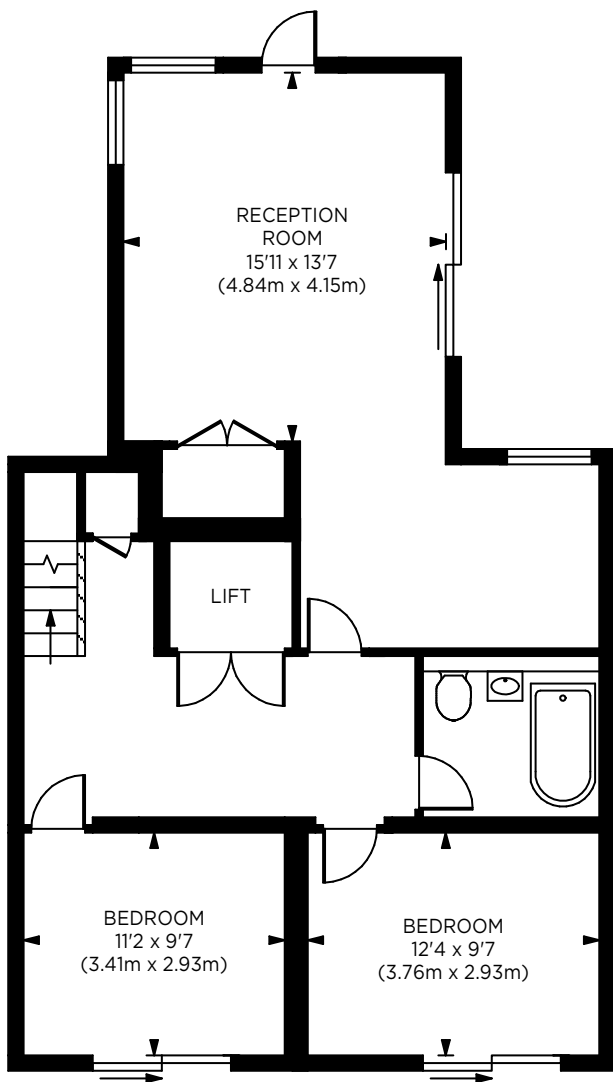
BASEMENT
